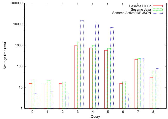
Figure 4: Querying Sesame ActiveRDF using JSON
