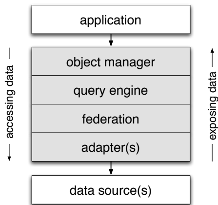
Figure 1: ActiveRDF architecture
